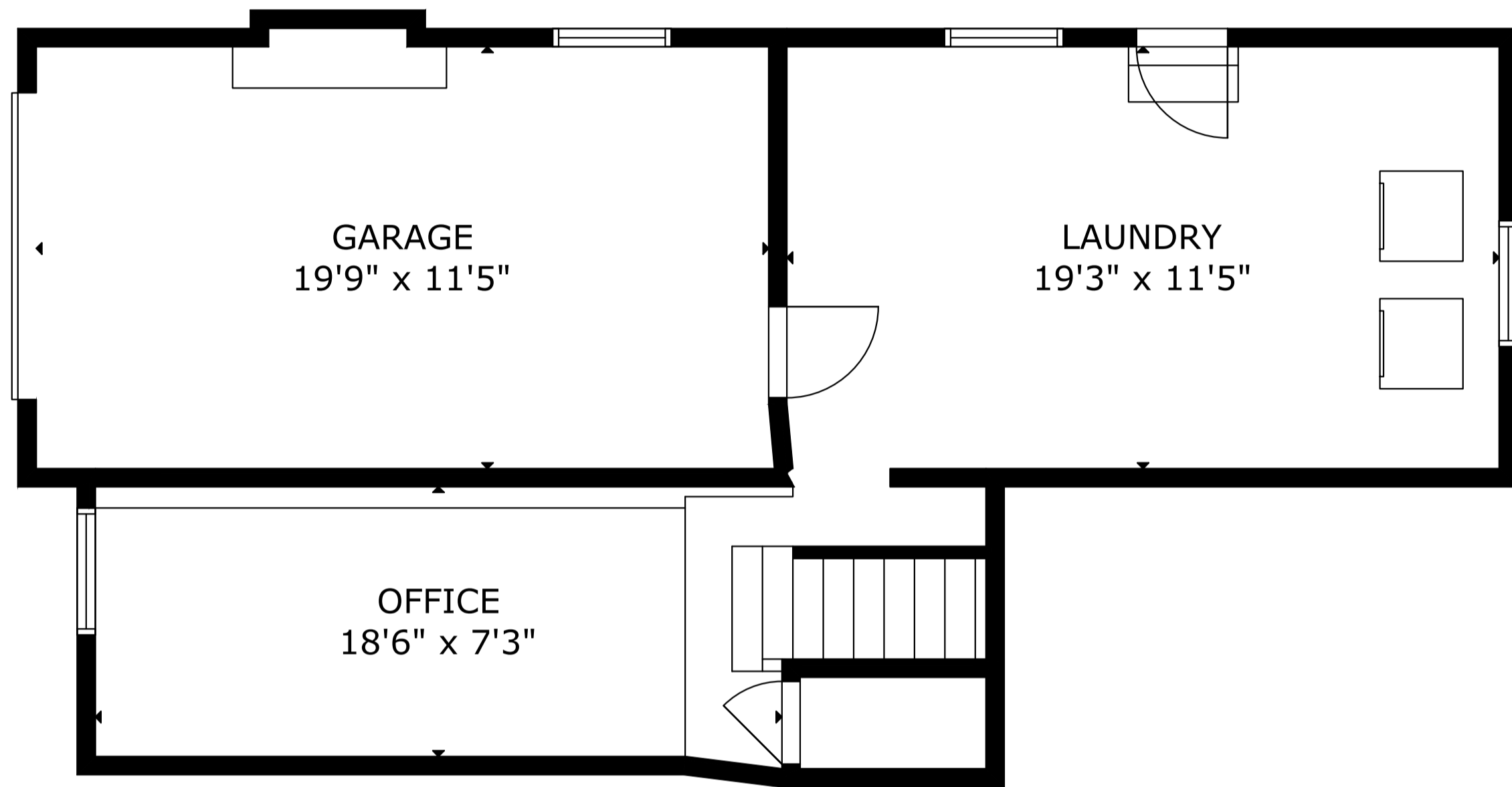
FLOOR 1
